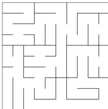
Figure 366: How the Recursive Division Algorithm Works (6/6)
